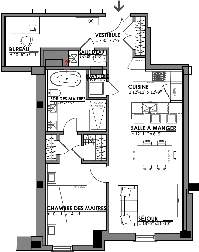
ÉCHELLE: 3/8" = 1'-0"
